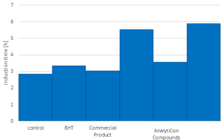
Induction time of different compounds at 110°C in flaxseed oil.
